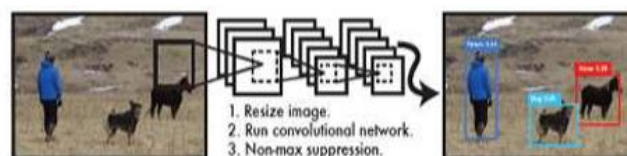
Fig. 1. The YOLO Detection System Processing images
