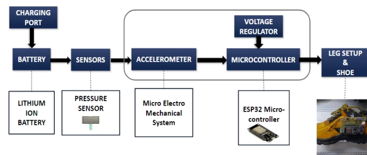
Fig. 2. Transmitting Shoe work flow
